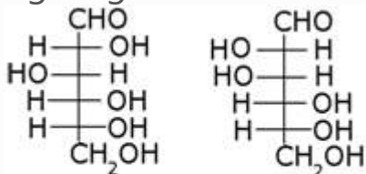
D - Glucose
